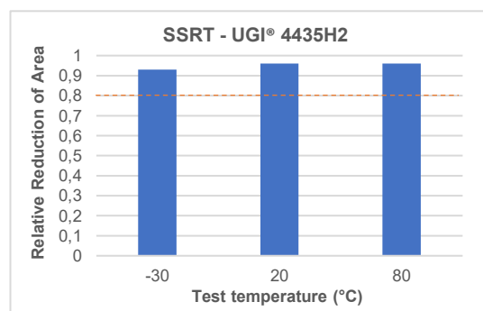
Slow strain rate test results under 100 bar H 2 / air
